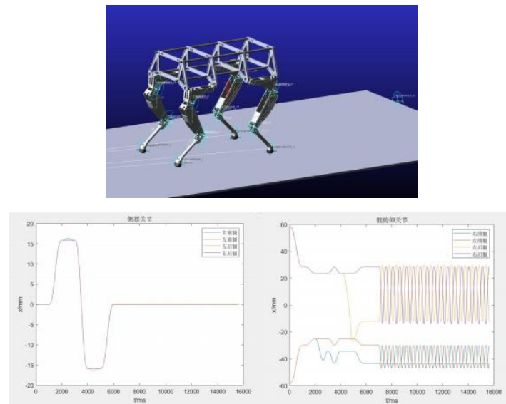
Fig.5 ADAMS simulation and quadruped joint planning trajectory diagram
